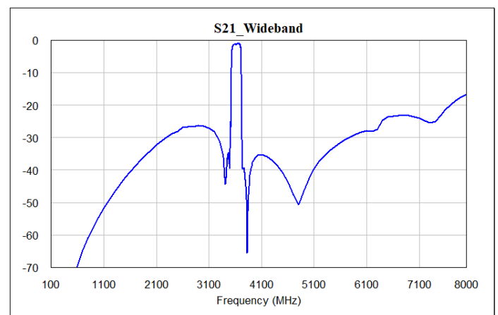
Wideband Response
