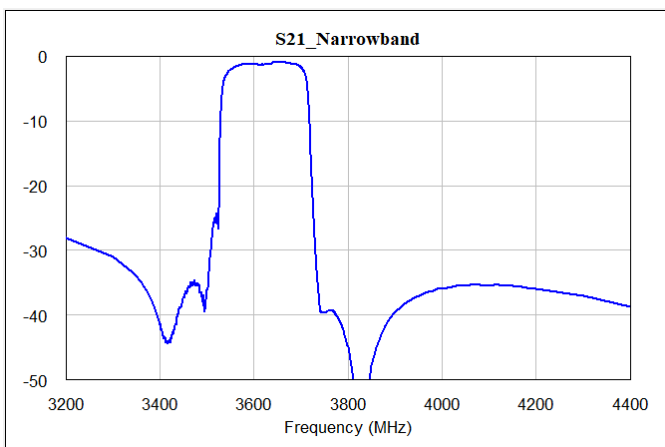
Narrowband Response
