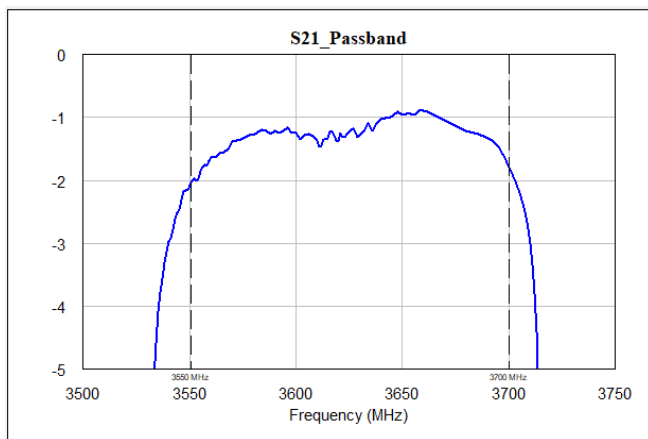
Passband Insertion Loss
