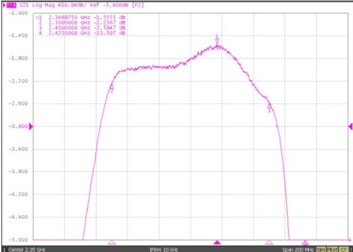
S21 response: (span 200MHz)
