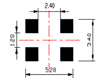
Recommended Solder Pattern
